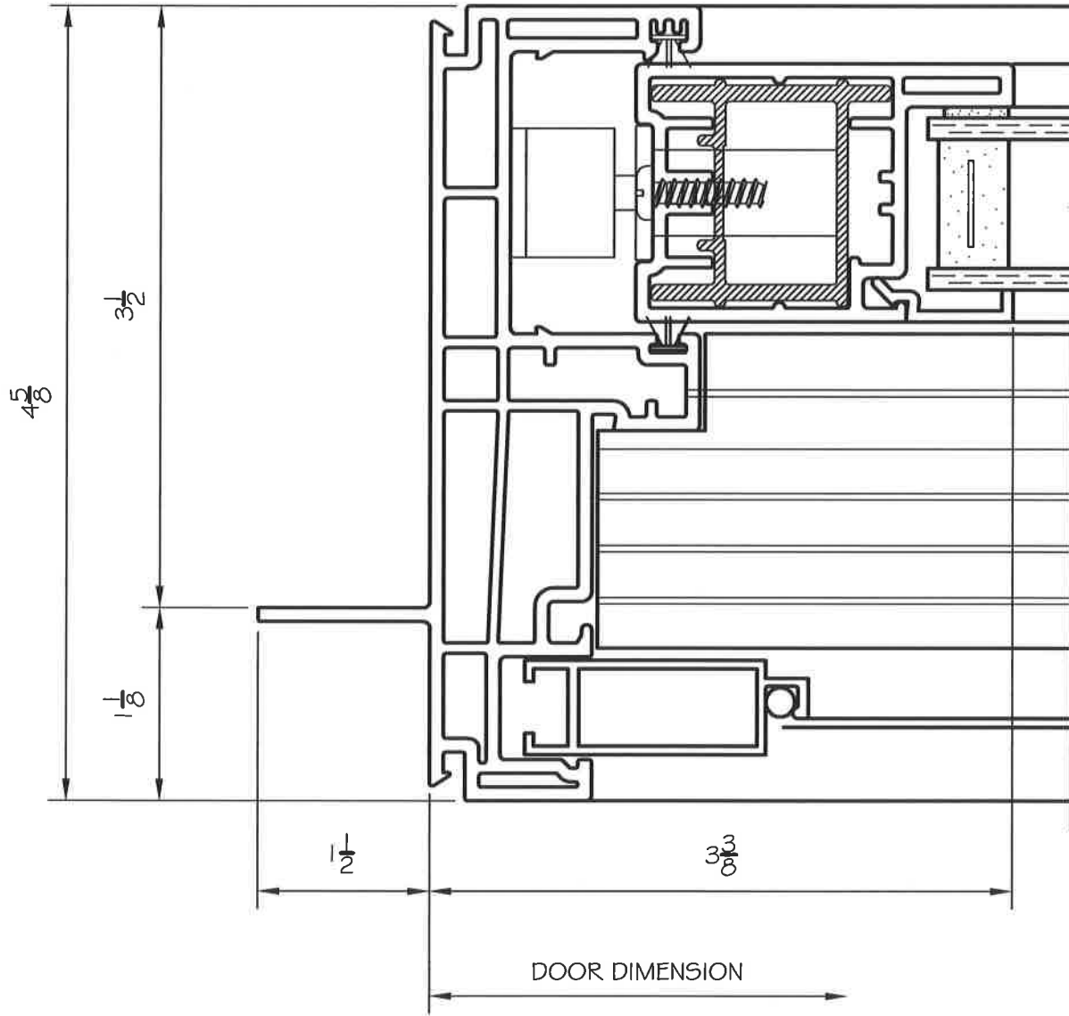
3 JAMB AT SASH
