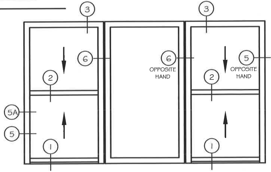
TYPICAL 2-LITE DOUBLE HUNG W/ ROUND TOP
