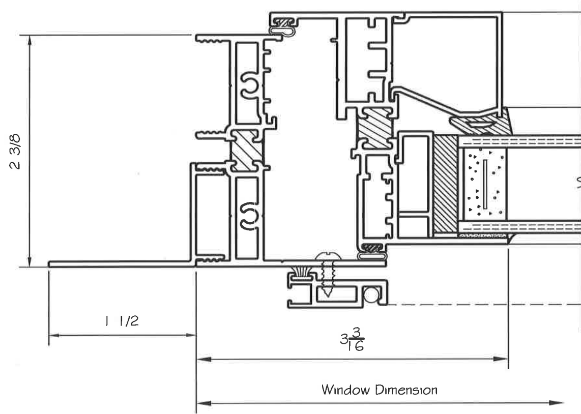
5 JAMB AT SASH W/ OPTIONAL NAILING FLANGE
