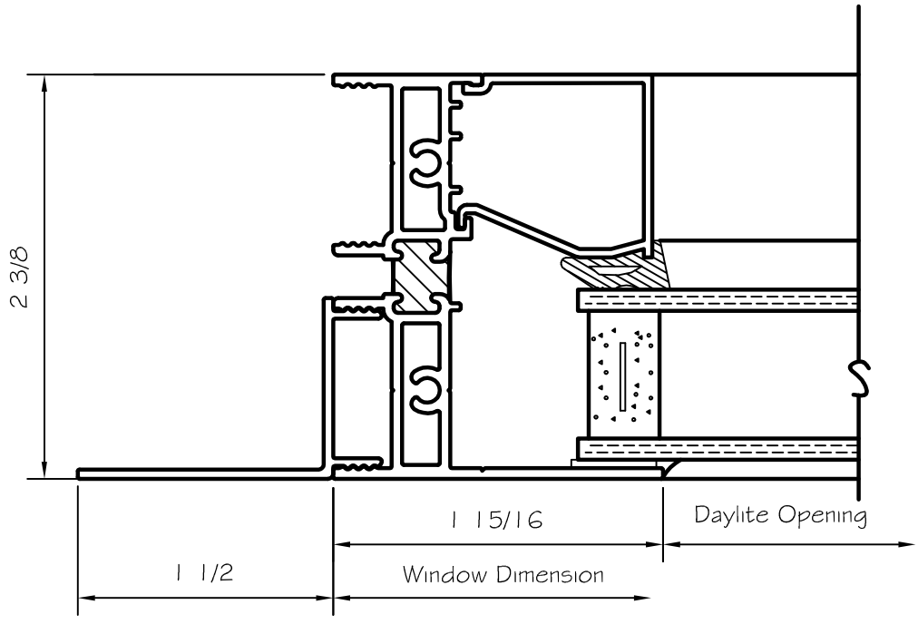
7 JAMB AT FIXED W/ OPTIONAL NAILING FLANGE
