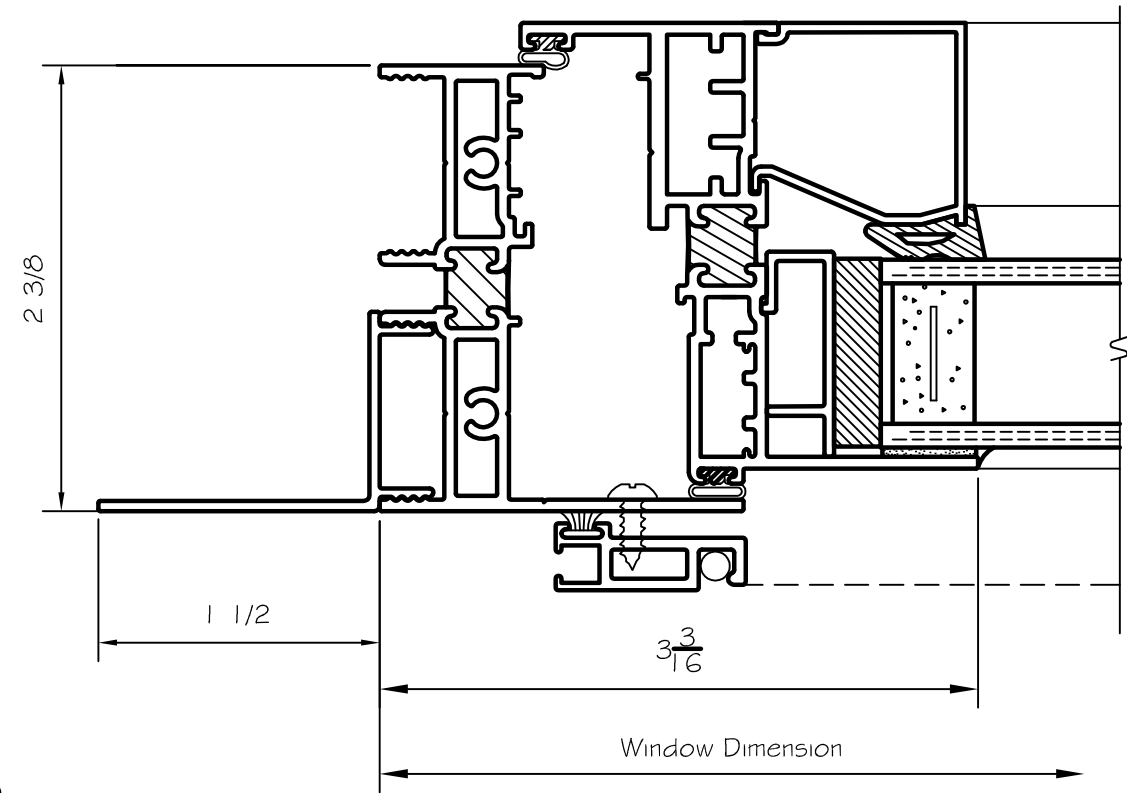
5 JAMB AT SASH W/ OPTIONAL NAILING FLANGE
