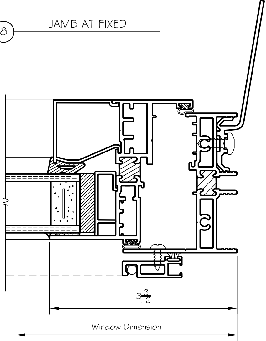
6 JAMB AT SASH W/ OPTIONAL STRAP ANCHOR
