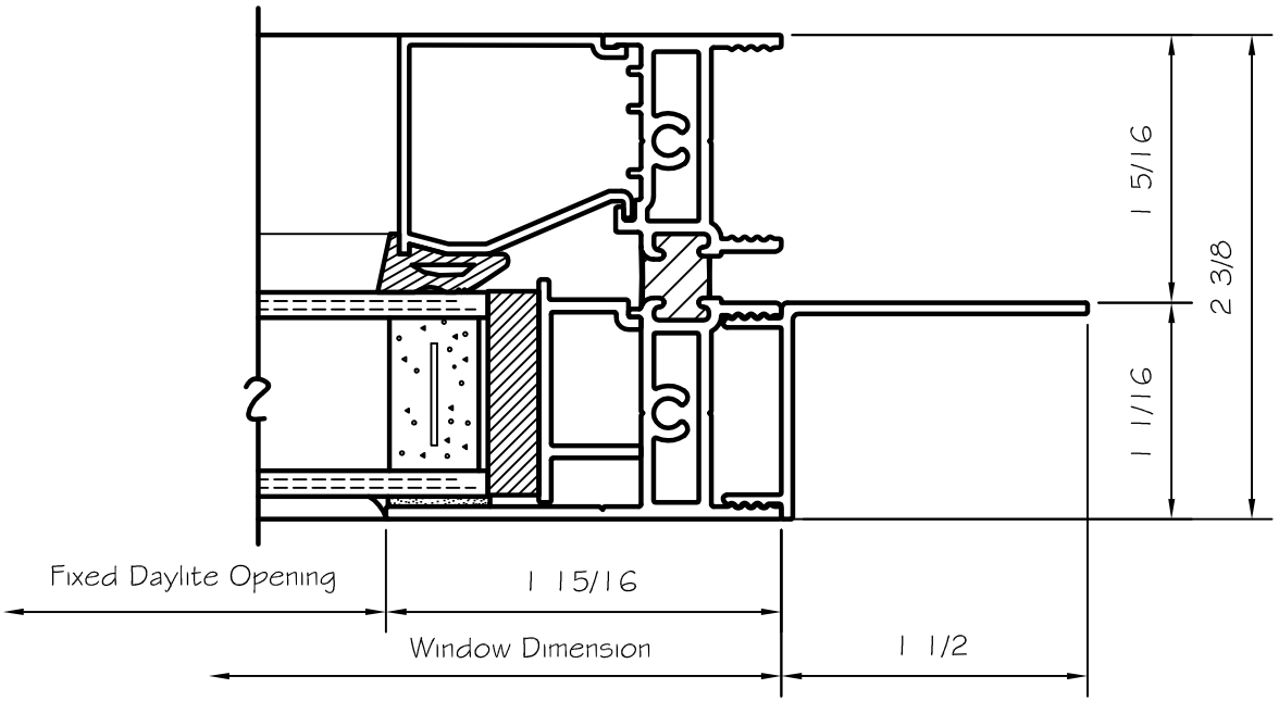
8 JAMB AT FIXED
