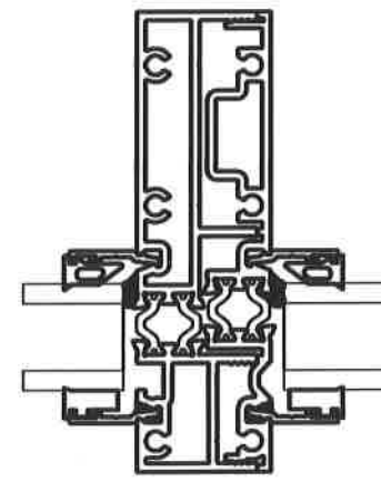
Stacking True Muntin 99" tall at 60" on center AAMA Rating LC-PG50 or CW-PG45
