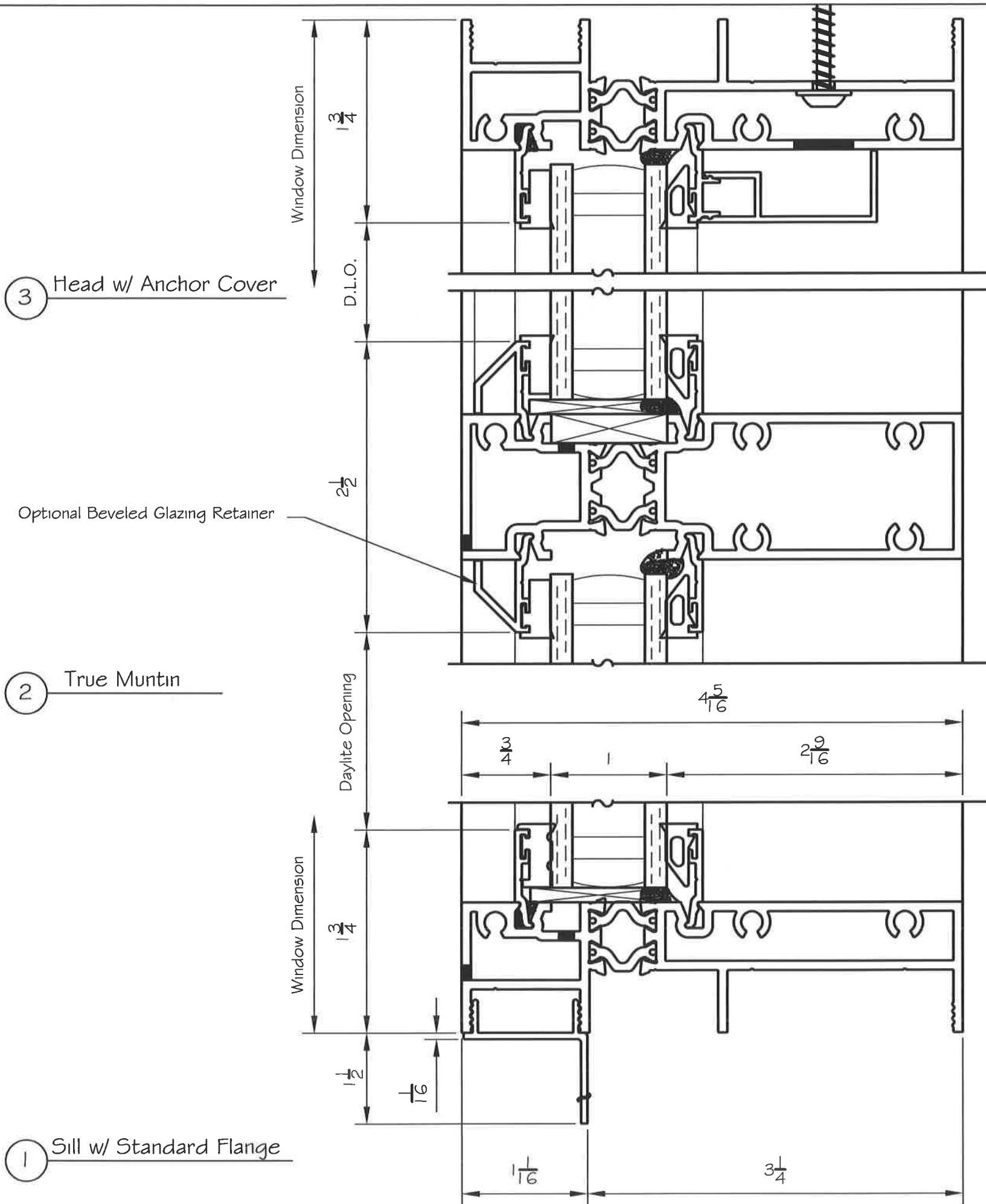
Stacking True Muntin 99" tall at 60" on center AAMA Rating LC-PG50 or CW-PG45
