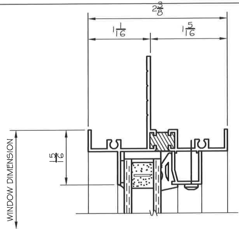
5 HEAD AT ROUND TOP
