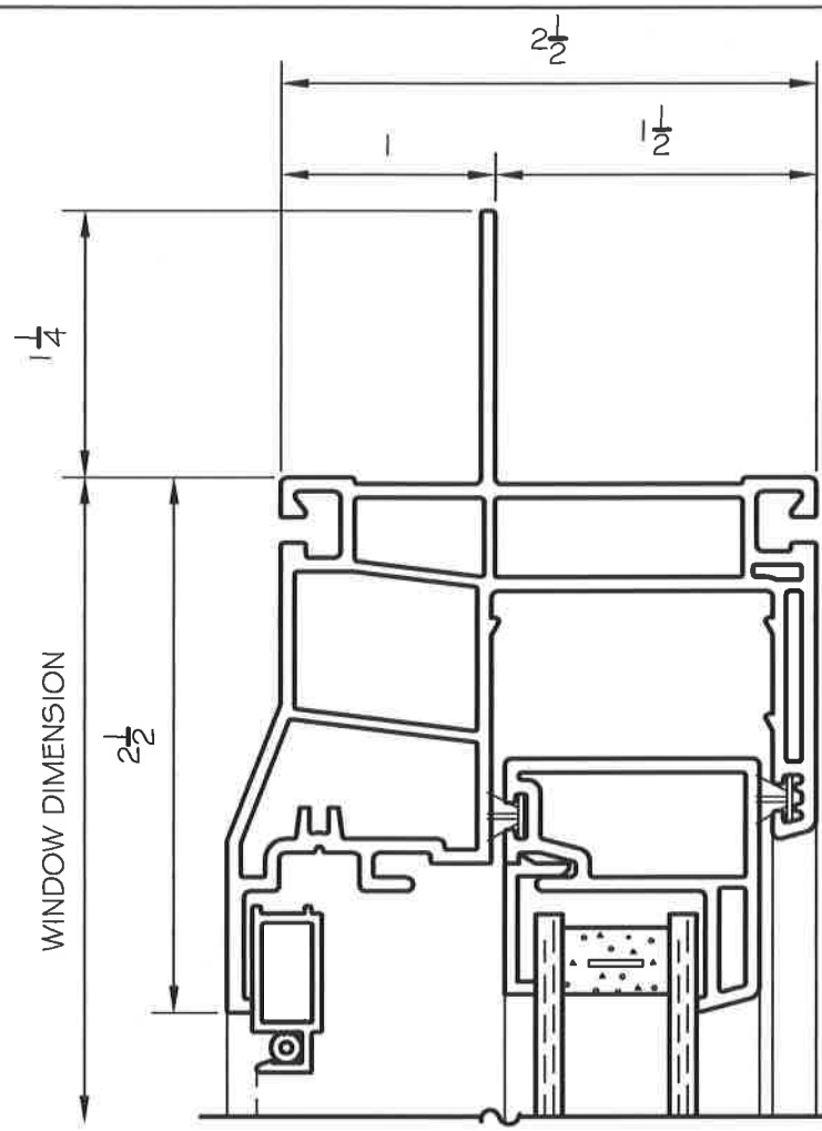
2 TYP. HEAD AT FIXED LITE
