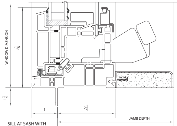
1 SILL AT SASH WITH OPTIONAL EXTENSION JAMB
