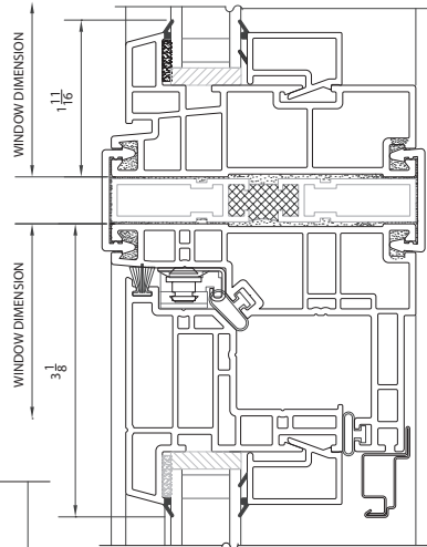
3 TYPICAL MULLION
