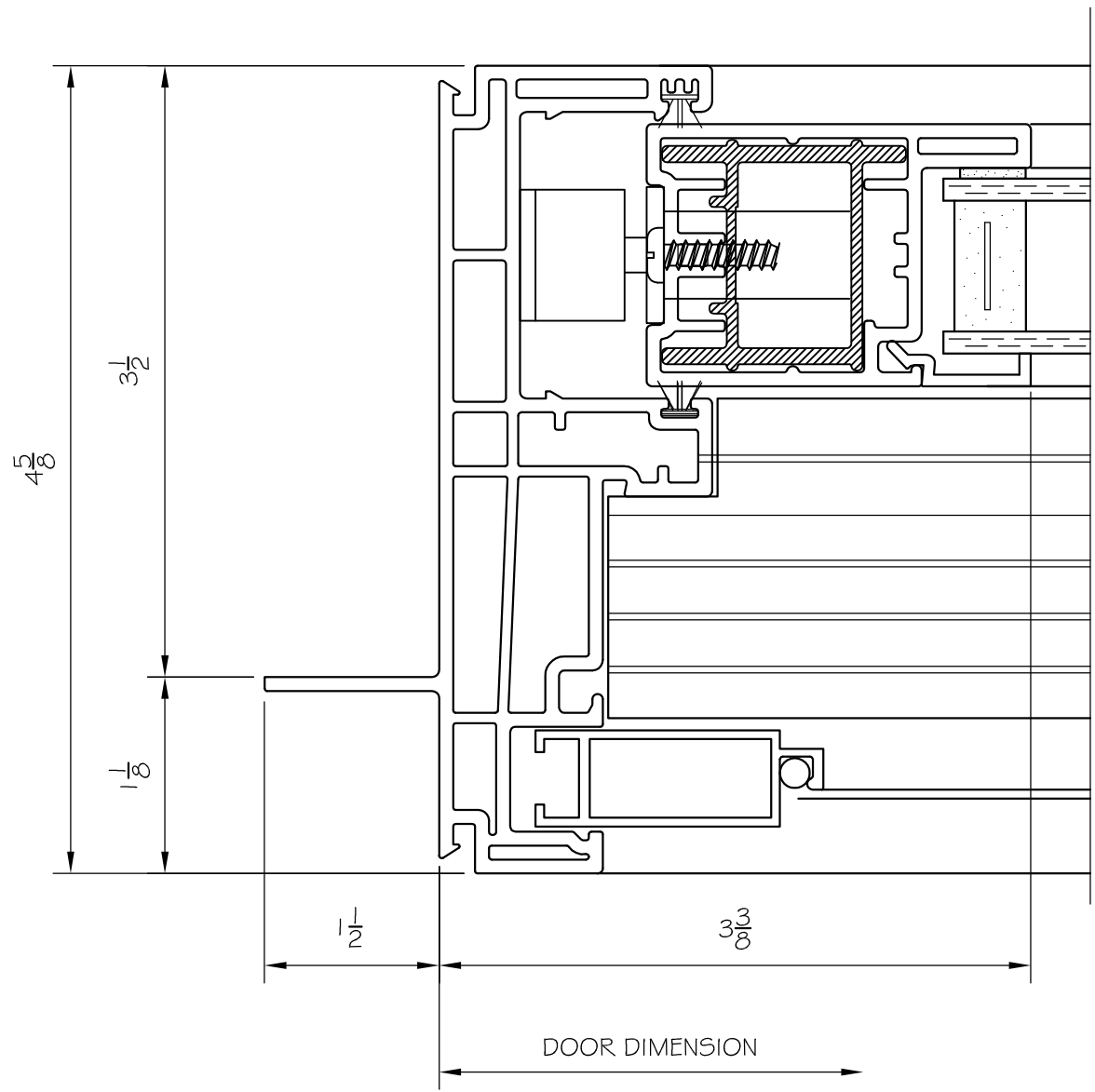
3 JAMB AT SASH
