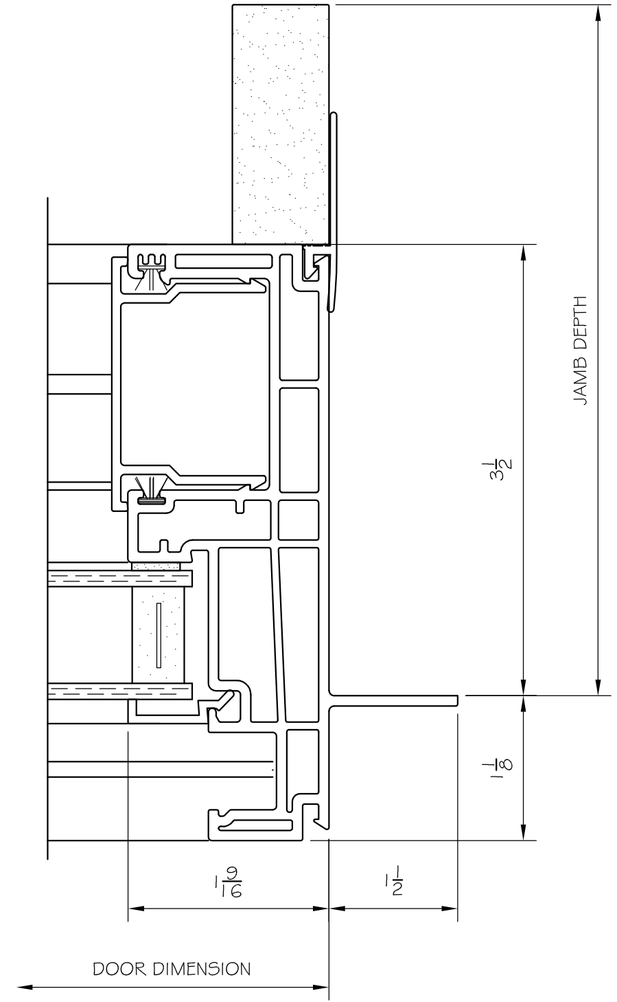
5 JAMB AT FIXED W/ OPTIONAL EXTENSION JAMB
